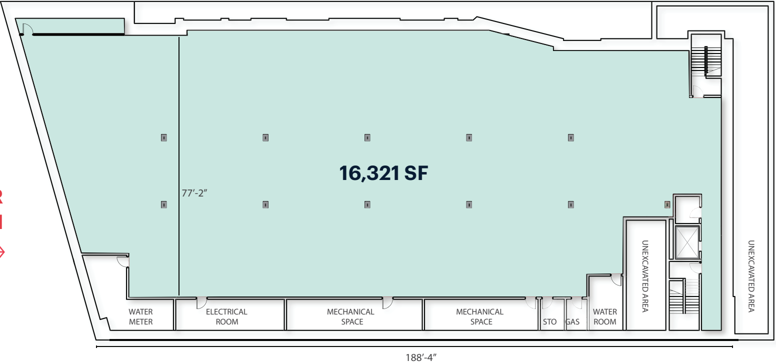
CELLAR FLOOR PLAN
